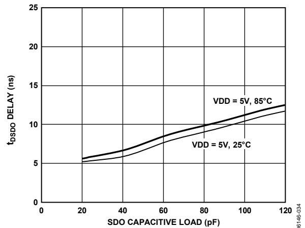
Figure 24. t_{0SDO} Delay vs. Capacitance Load and Supply
